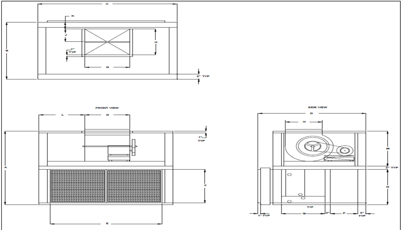
Dimension Table
