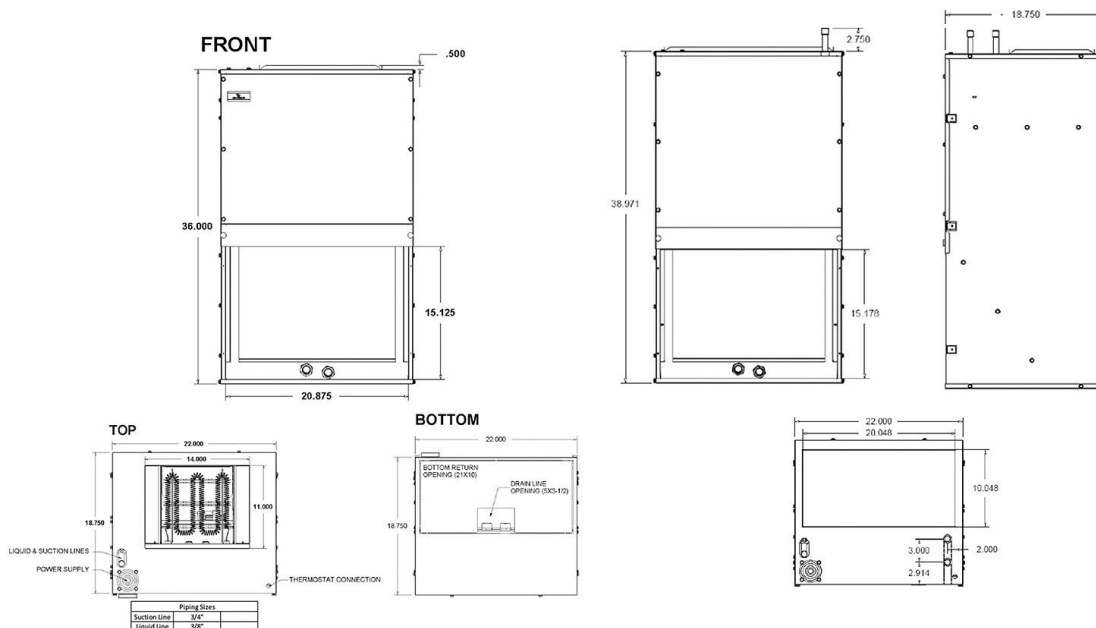
Unit Dimensional Data AHW1
