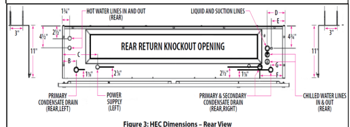
Figure 3: HEC Dimensions - Rear View
