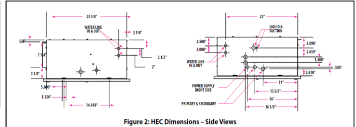
Figure 2: HEC Dimensions - Side Views
