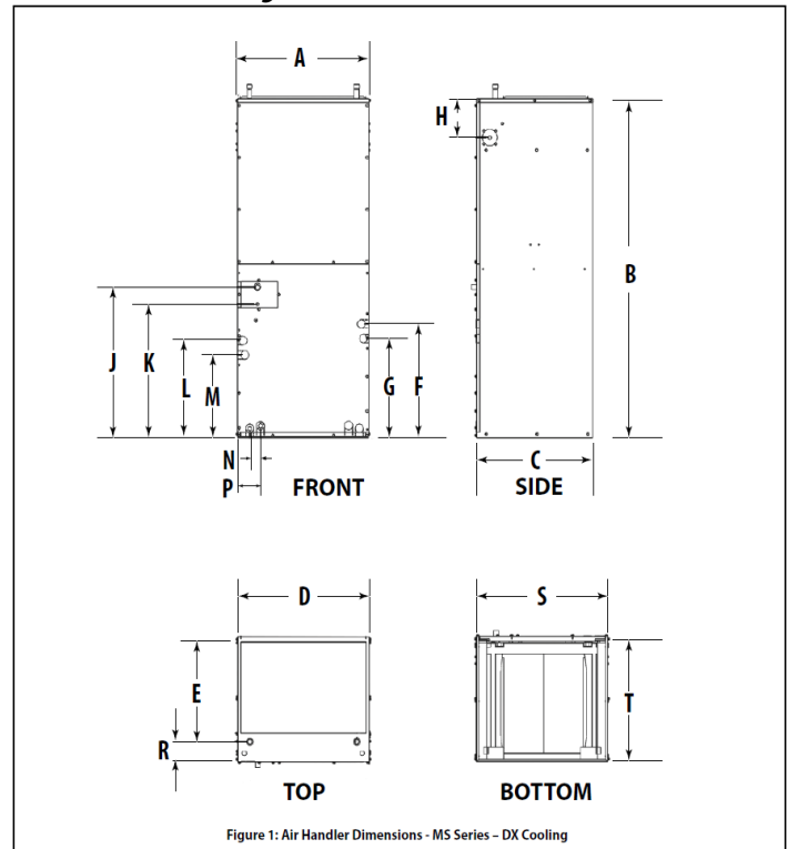
Figure 1: Air Handler Dimensions - MS Series - DX Cooling
